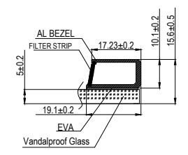
Section A-A Detail 5:1
