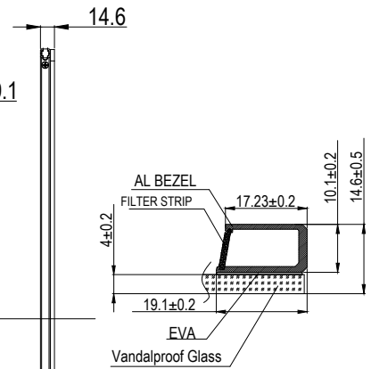
Section A-A Detail 5:1
