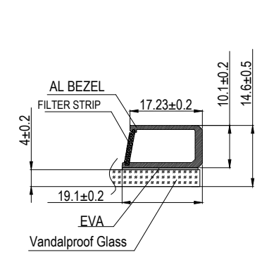
Section A-A Detail 5:1
